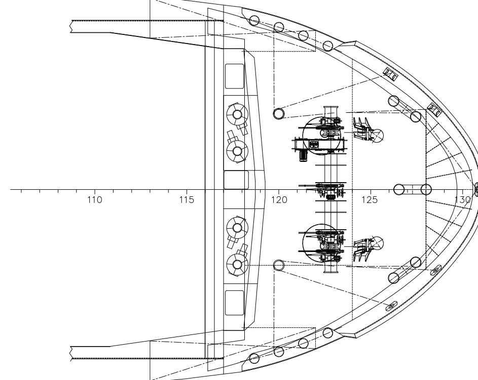
FORE CASTLE
