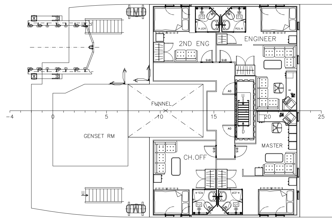
BOAT DECK
