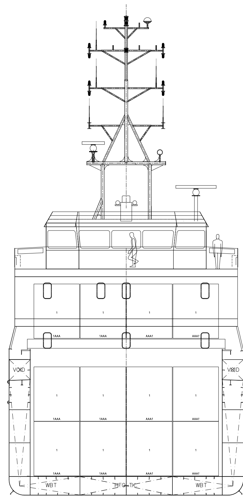
CROSS SECTION
