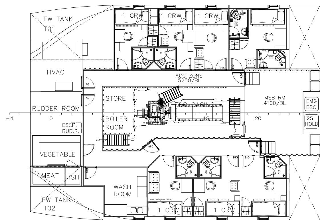
MAIN DECK
