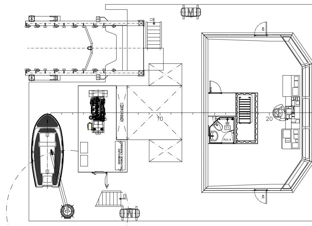
BRIDGE DECK
